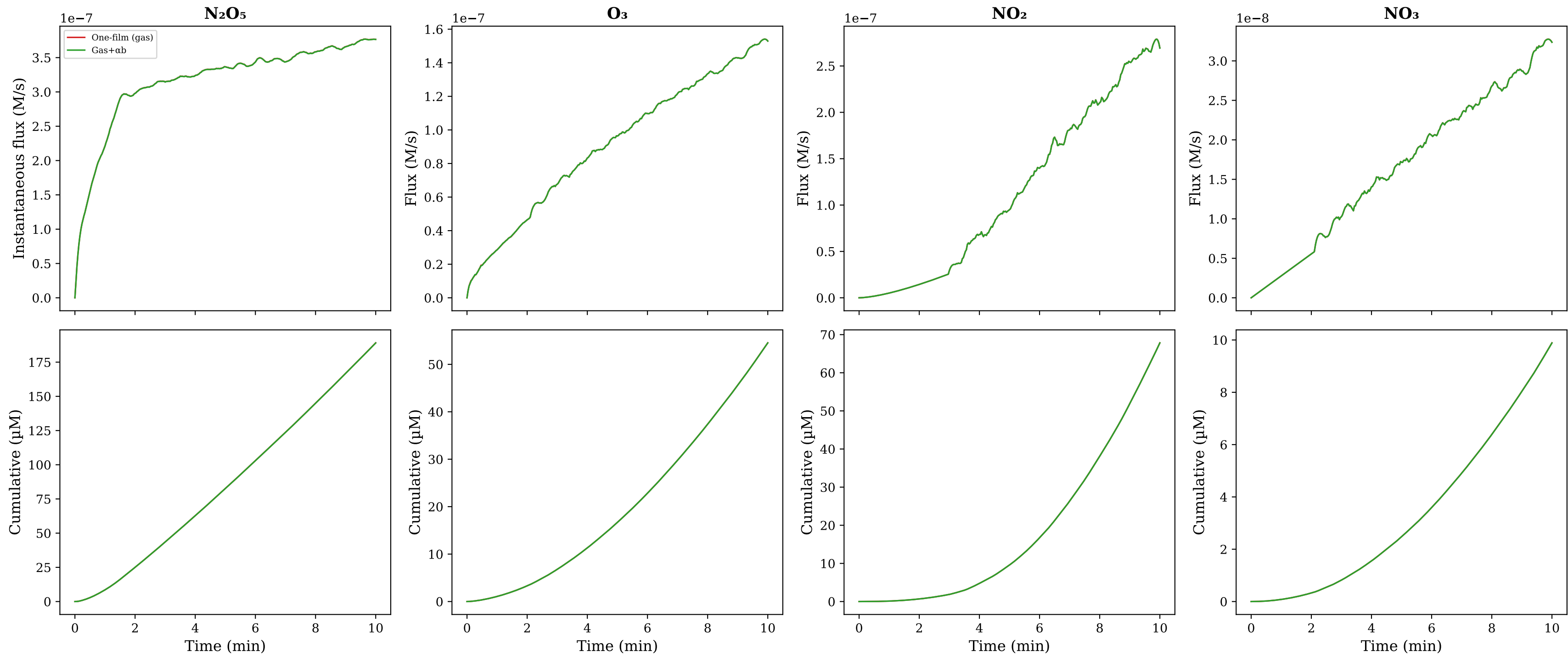
Mass transfer flux by BC type (DIW, 600 s)
